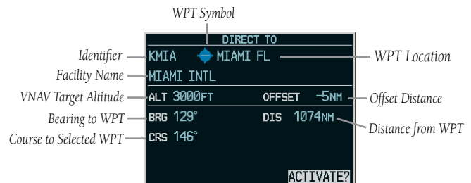
Figure 7-7 PFD Direct-to Window
