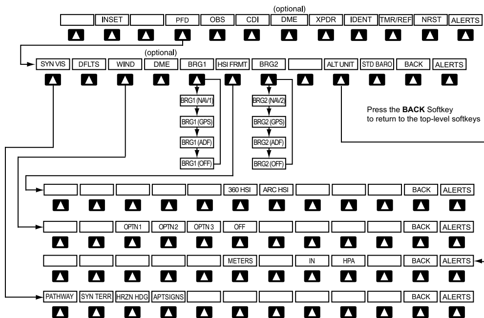
Figure 1-3 PFD Configuration Softkeys
