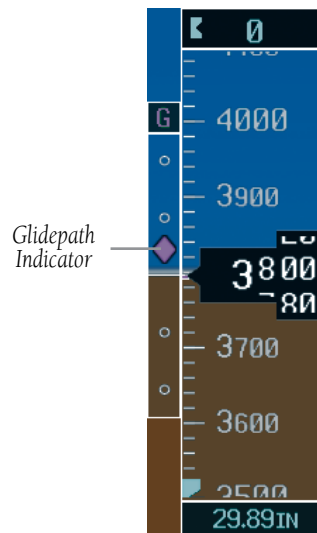
Figure 2-12 Glidepath Indicator
