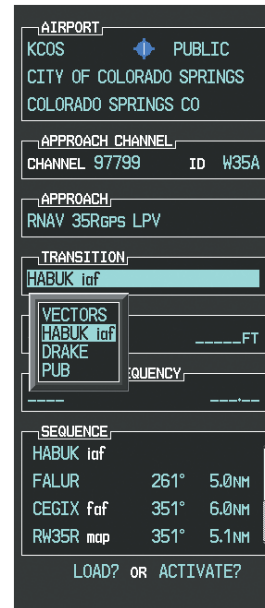
Figure 7-32 List of Available Transitions
