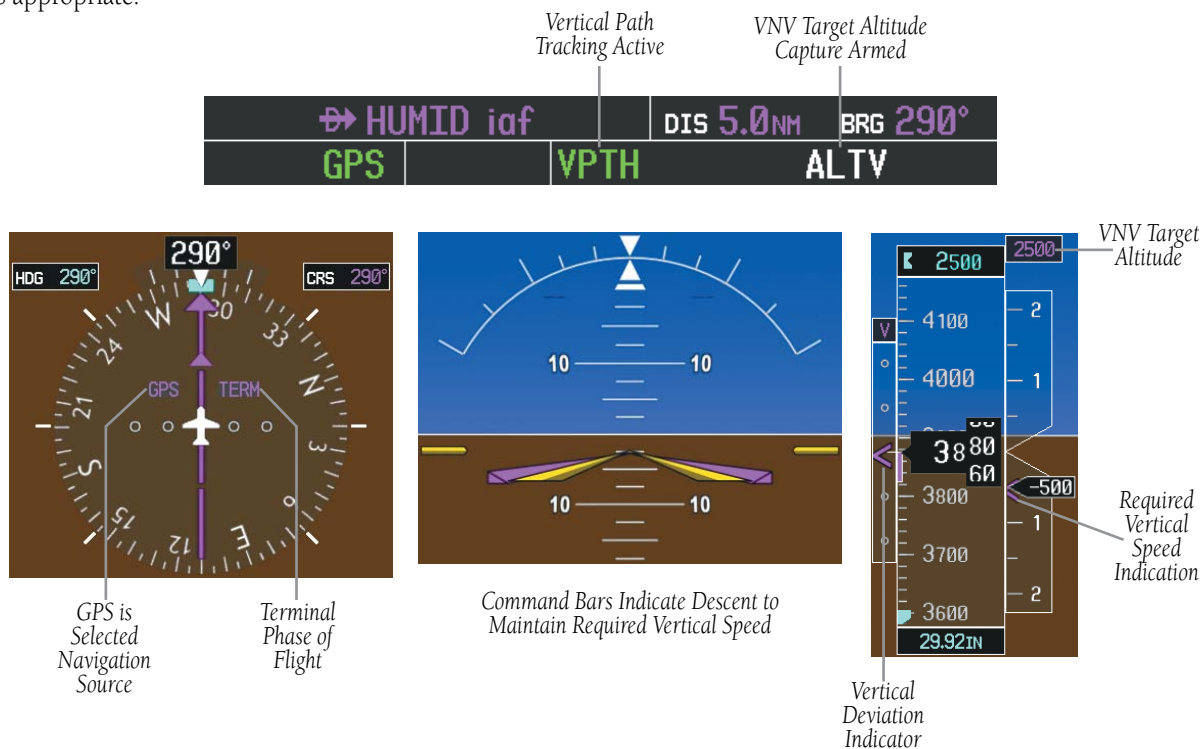
Figure 6-12 Vertical Path Tracking Mode
