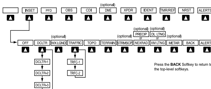
Figure 1-2 INSET Softkeys
