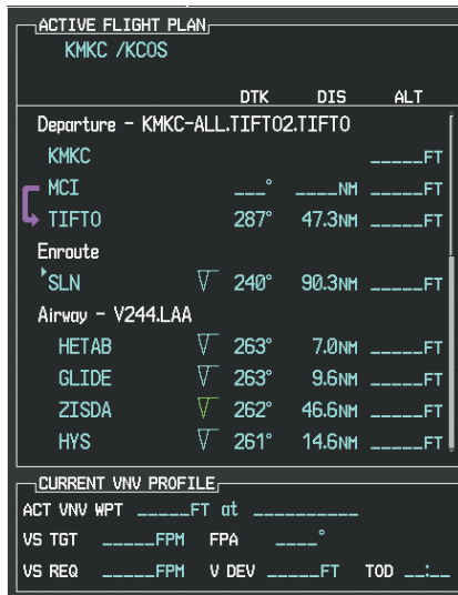
Figure 7-13 Begin Adding V4 to the Flight Plan
