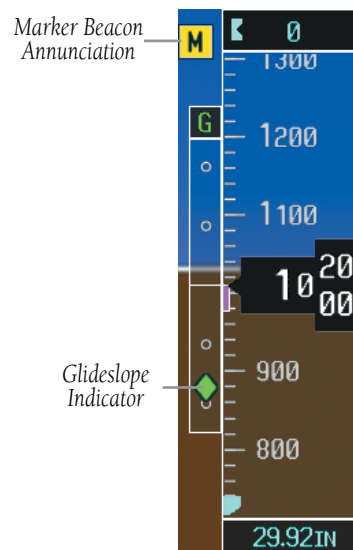
Figure 2-13 Glideslope Indicator
