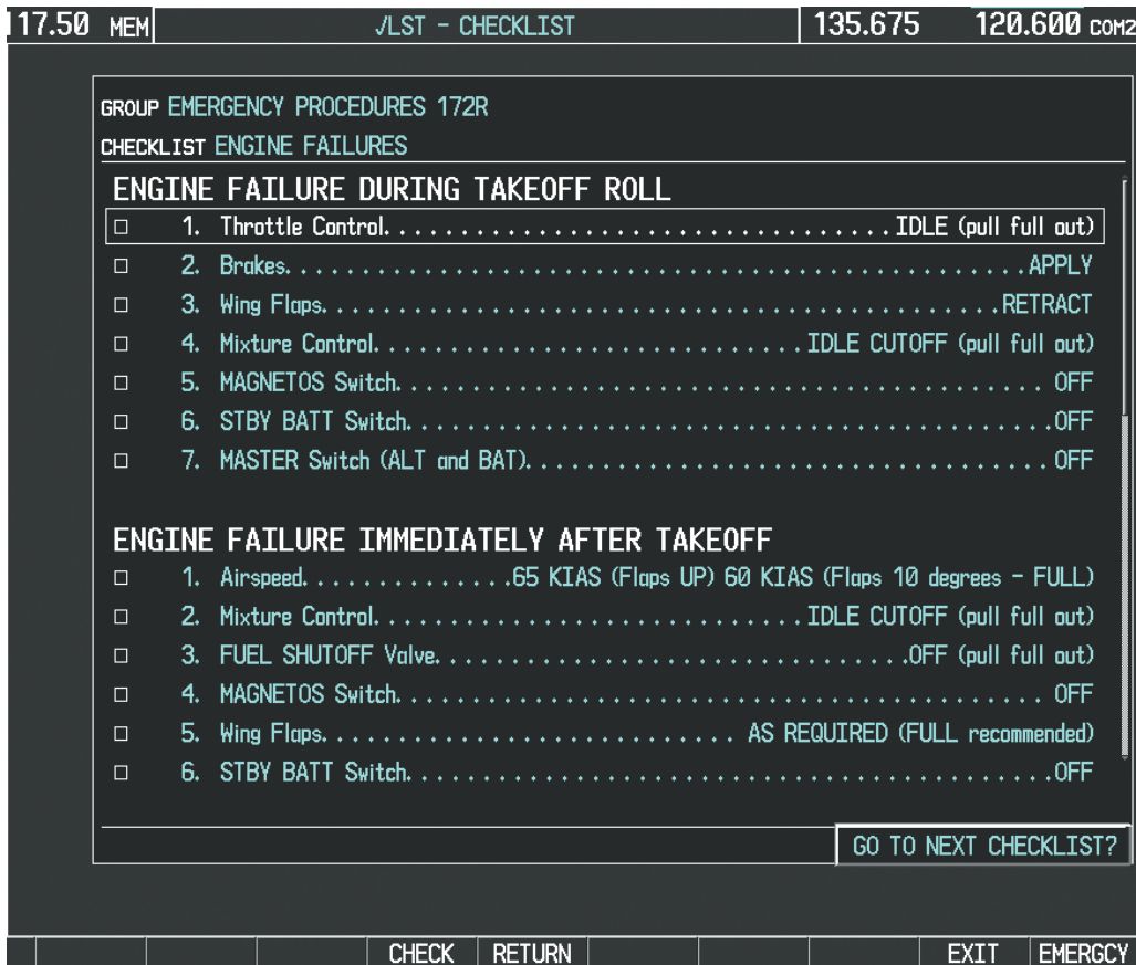
Figure 11-33 Emergency Checklist Page Example
