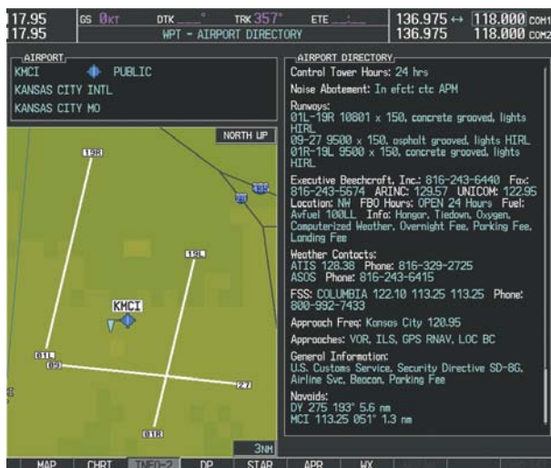
Figure 7-53 AOPA Airport Directory Information
