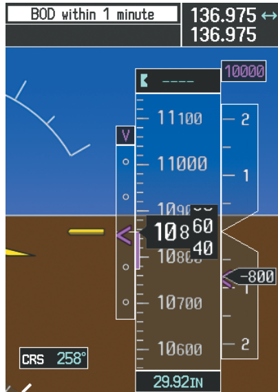
Figure 7-40 Approaching Bottom of Descent (BOD) at OPSHN Offset Waypoint
