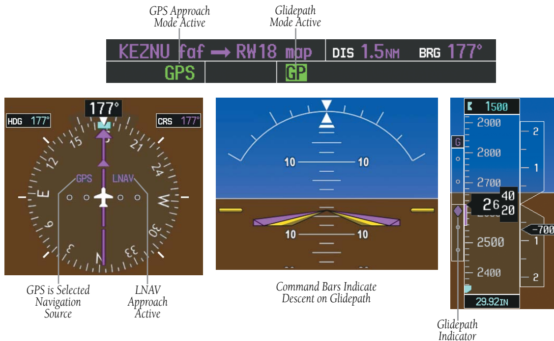
Figure 6-15 Glidepath Mode
