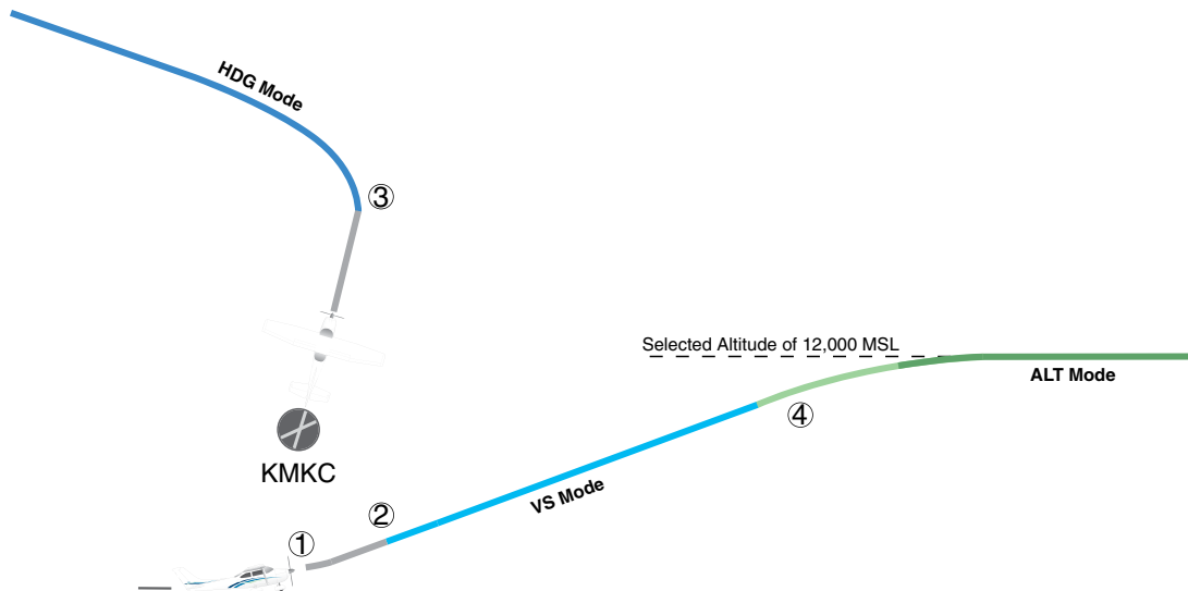
Figure 6-31 Departure
