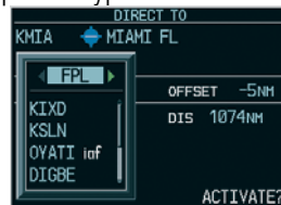
Figure 7-8 Flight Plan Waypoint List (PFD)
