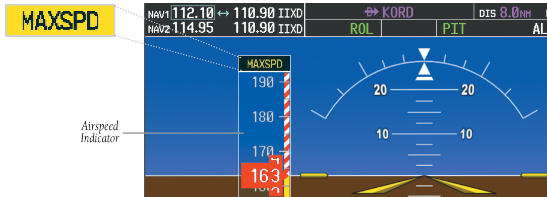
Figure 6-41 Overspeed Annunciation
