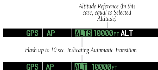
Figure 6-6 Automatic Mode Transitions During Altitude Capture
