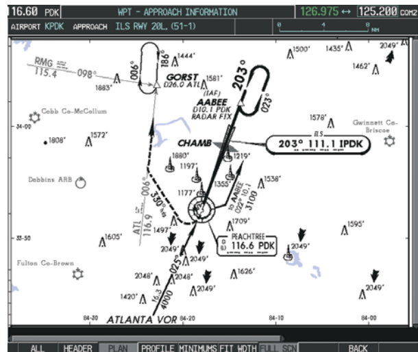
Figure 11-19 Approach Information Page, Plan View
