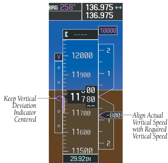
Figure 7-39 VDI & RVSI Showing Correctly Established Descent
