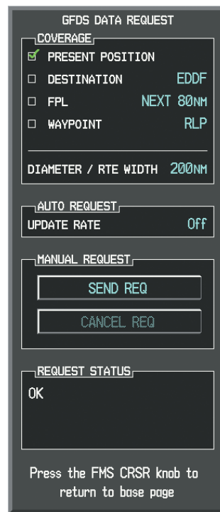
Figure 10-23 GFDS Data Request Window
