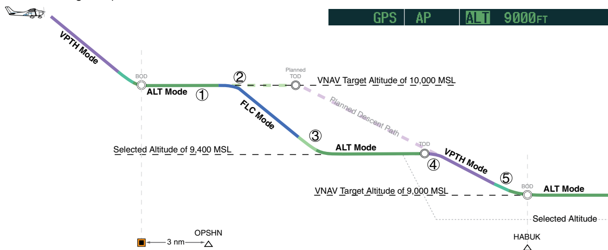
Figure 6-36 Non-path Descent
