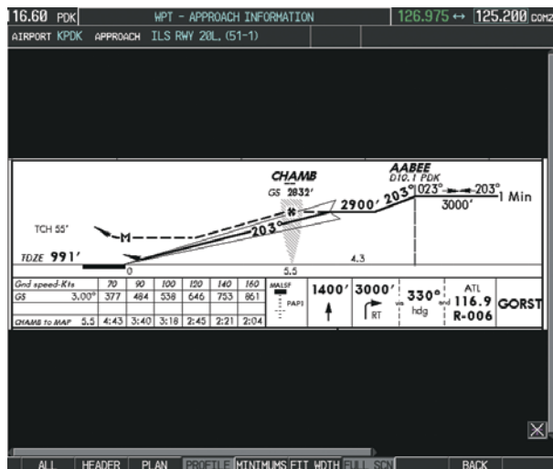
Figure 11-20 Approach Information Page, Profile View
