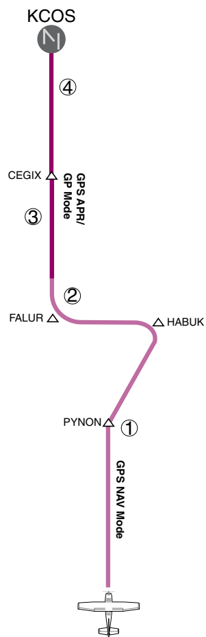
Figure 6-38 LPV Approach to KCOS
