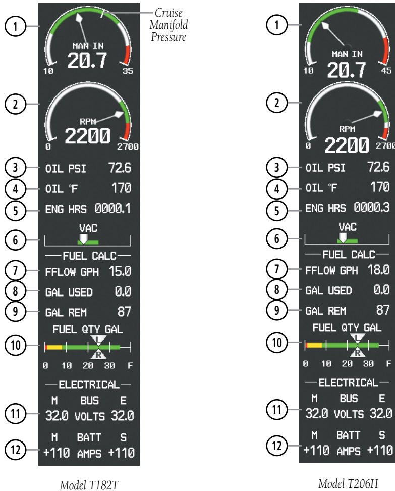
Figure 3-6 System Display (Turbocharged Aircraft)
