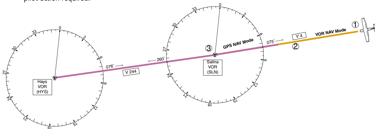
Figure 6-33 Transition to GPS Flight Plan
