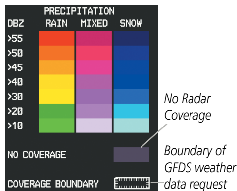
Figure 10-29 Precipitation Data Legend
