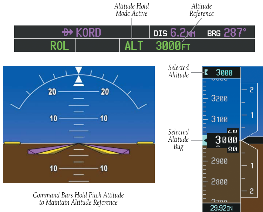
Figure 6-7 Altitude Hold Mode
