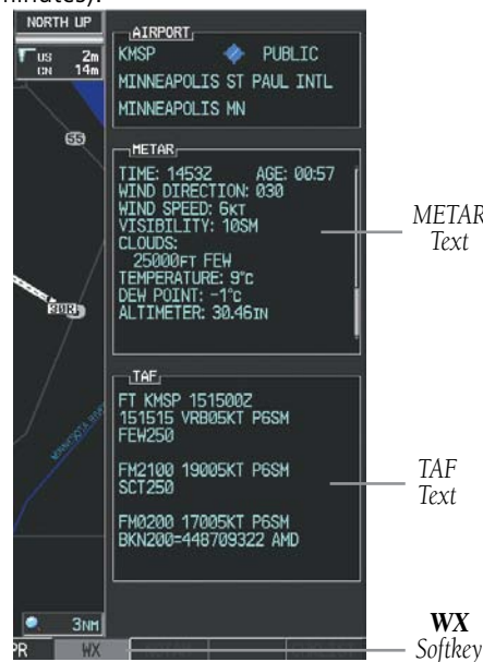
Figure 10-7 METAR and TAF Text Displayed on the Airport (Weather) Information Page
