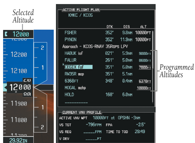
Figure 11-3 Programmed and Selected Altitude
