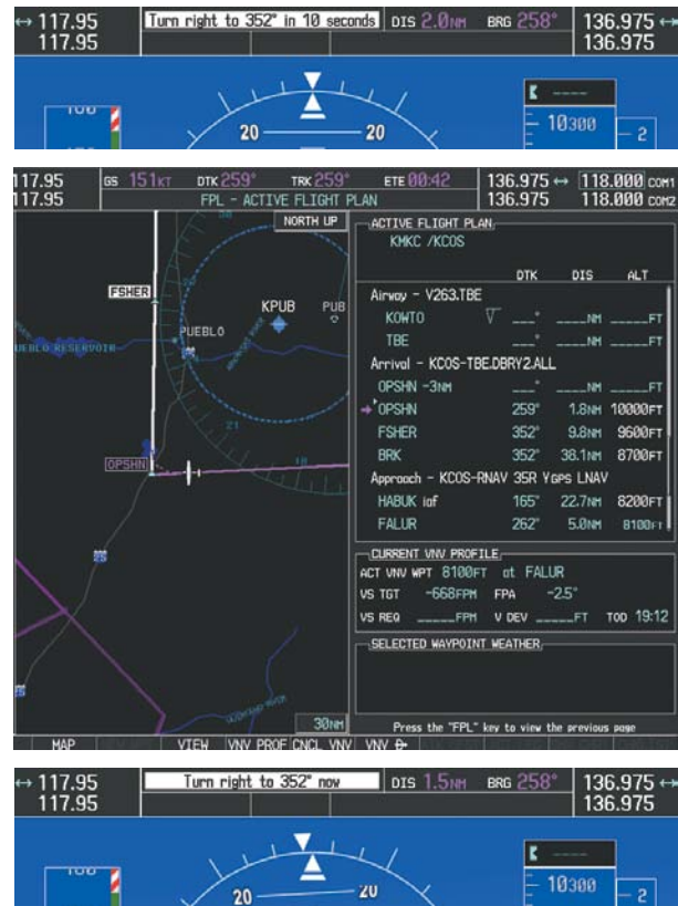
Figure 7-41 Turn to intercept OPSHN to FSHER Leg
