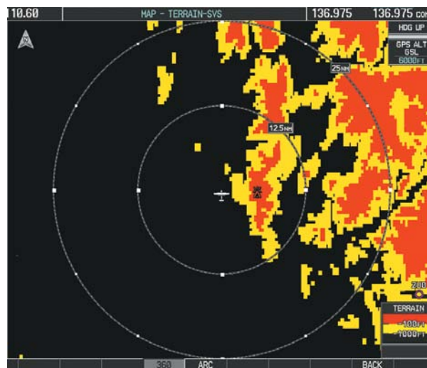
Figure 10-39 Terrain-SVS Page (360° View)
