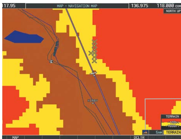
Figure 10-44 Navigation Map Page (After TERRAIN-SVS Pop-up Alert Acknowledgment)
