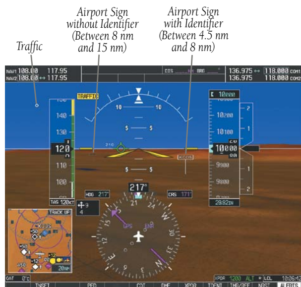
Figure 11-7 Airport Signs
