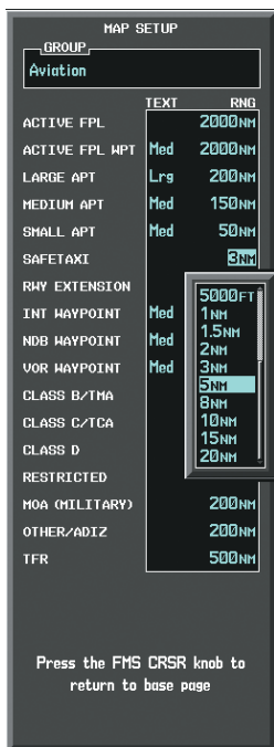
Figure 11-15 MAP SETUP Menu, Aviation Group
