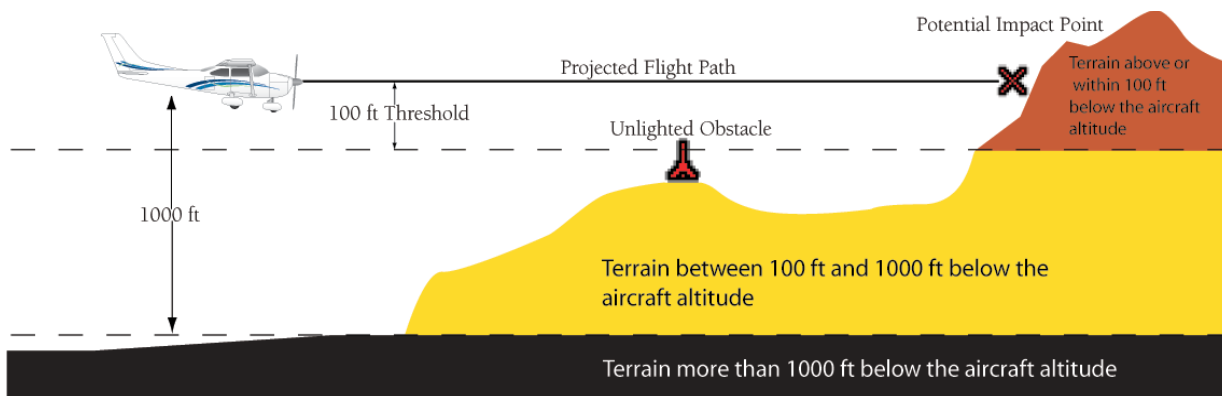
Figure 10-41 Terrain-Color Code
