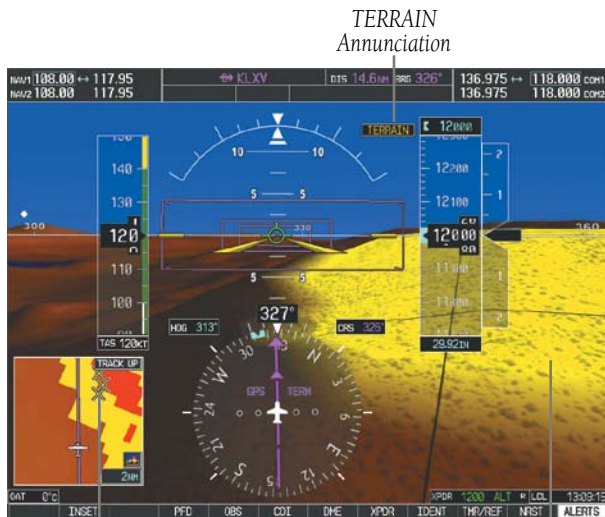
Figure 11-9 Terrain Alert
