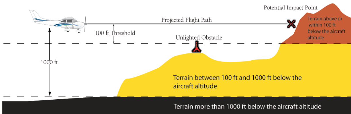
Figure 10-46 Terrain-Color Code
