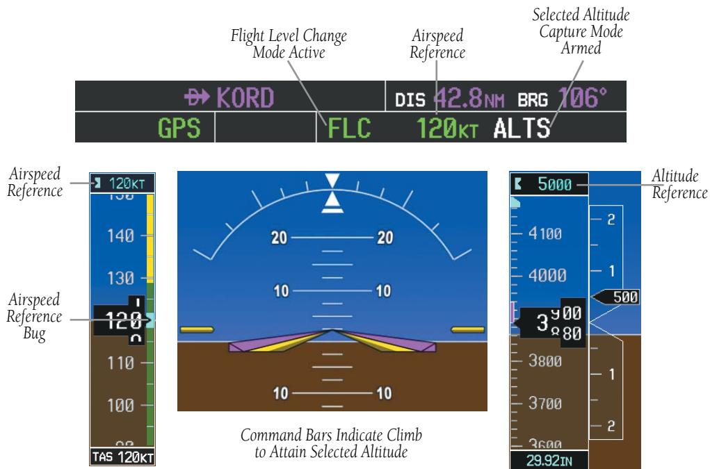
Figure 6-9 Flight Level Change Mode
