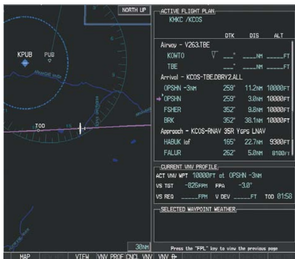
Figure 7-37 Approaching Top of Descent (TOD)
