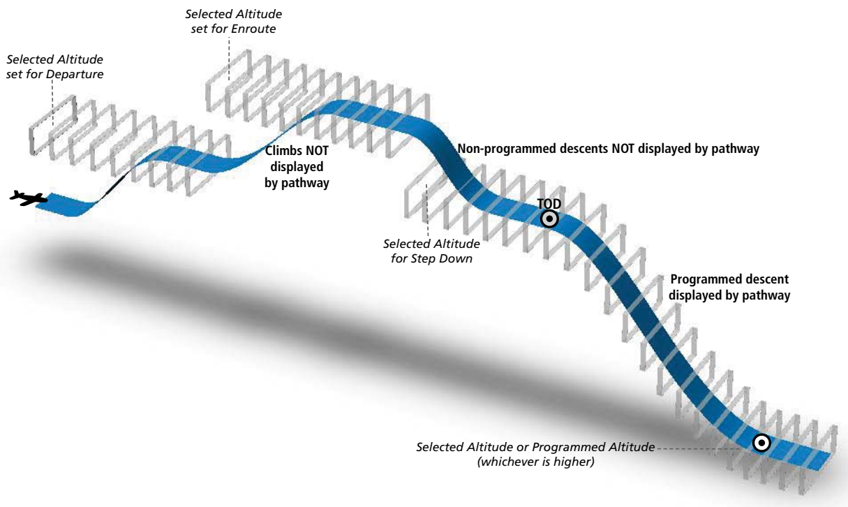
Figure 11-4 SVS Pathways, Enroute and Descent
