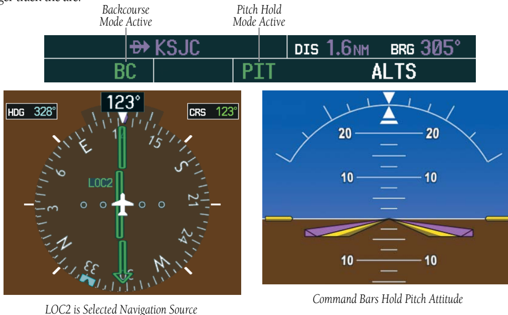
Figure 6-25 Backcourse Mode
