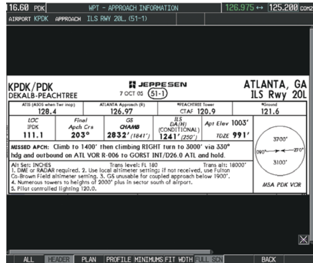
Figure 11-18 Approach Information Page, Header View
