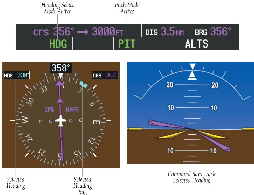
Figure 6-21 Heading Select Mode
