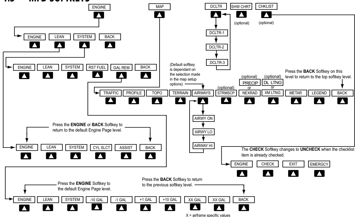
Figure 1-5 MFD Softkeys
