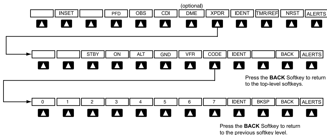
Figure 1-4 XPDR (Transponder) Softkeys
