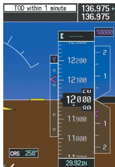
Figure 7-38 VDI & RVSI Upon Reaching Top of Descent (TOD)
