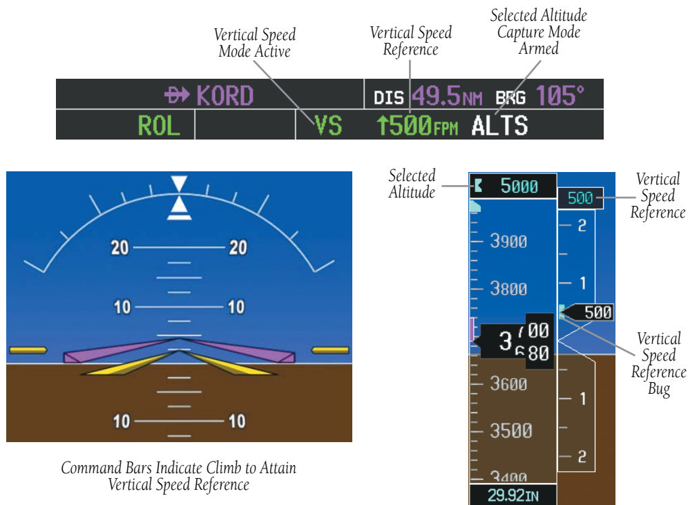
Figure 6-8 Vertical Speed Mode
