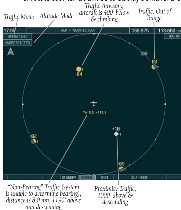
Figure 10-34 Traffic Map Page
