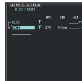
Figure 8-15 Airway Insertion Point
