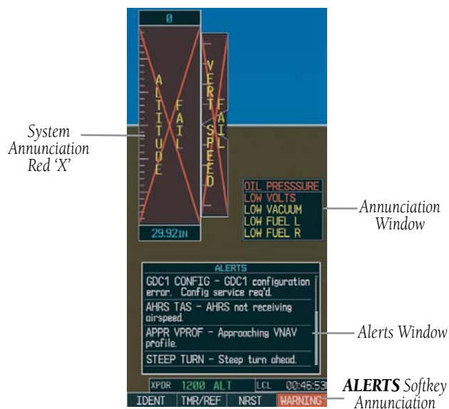
Figure 13-1 G1000 Alerting System
