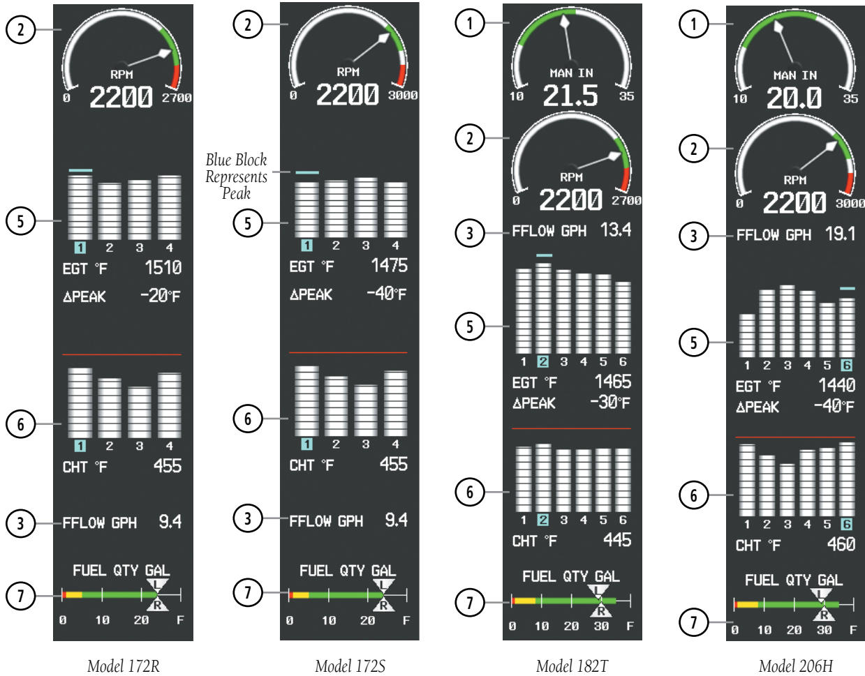
Figure 3-3 Lean Display (Normally-aspirated Aircraft)
