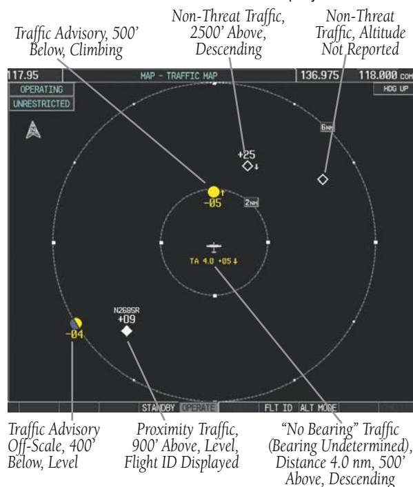
Figure 10-32 Traffic Map
