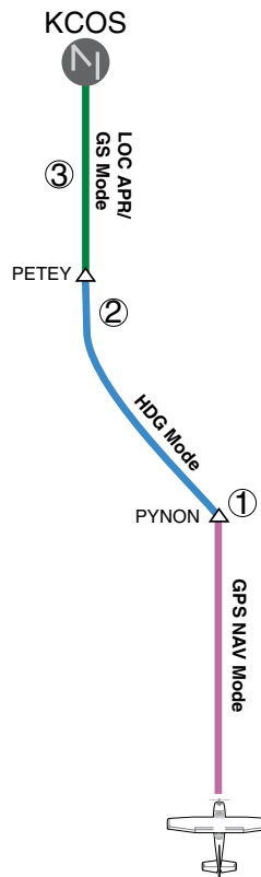
Figure 6-37 ILS Approach to KCOS
