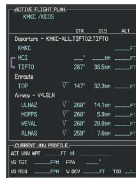
Figure 8-3 Active Flight Plan Page on the MFD
