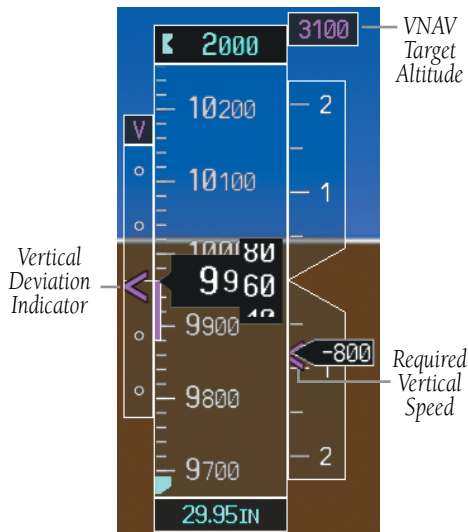
Figure 2-11 Vertical Deviation Indications
