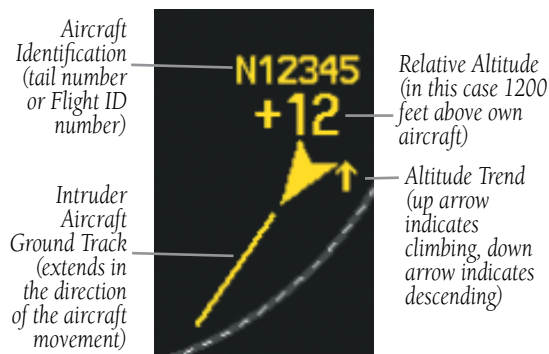
Figure 10-36 Example ADS-B Traffic Advisory
