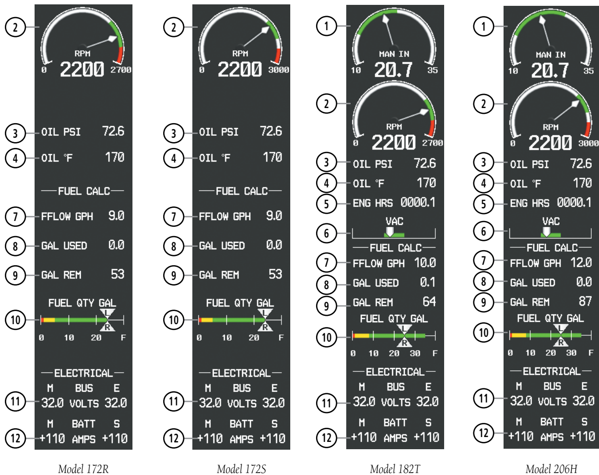
Figure 3-5 System Display (Normally-aspirated Aircraft)
