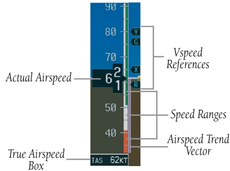
Figure 2-4 Airspeed Indicator
