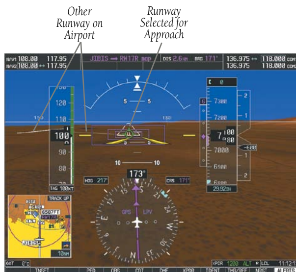
Figure 11-8 Airport Runways
