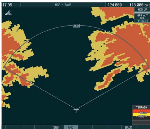
Figure 10-48 TAWS-B Page (ARC View)
