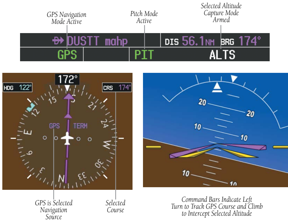
Figure 6-22 Navigation Mode
