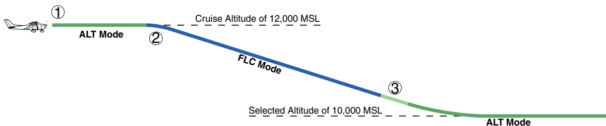
Figure 6-34 FLC Descent
