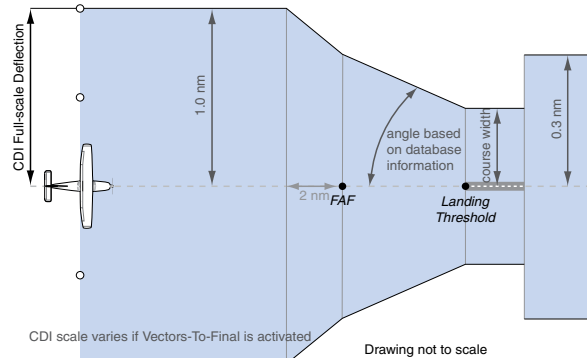
Figure 2-24 Typical LNAV/VNAV and LPV Approach CDI Scaling (SBAS Systems Only)
