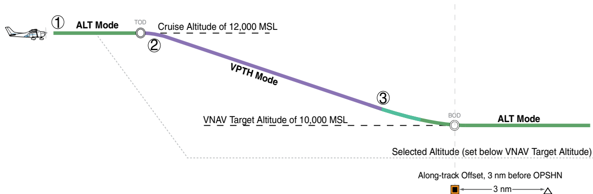
Figure 6-35 VPTH Descent
