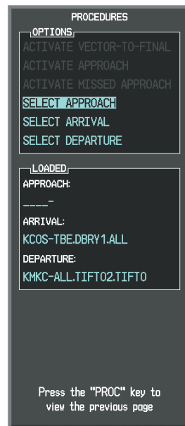
Figure 7-30 Procedures Window
