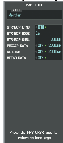
Figure 10-21 Navigation Map Page Setup Menu, Weather Group
