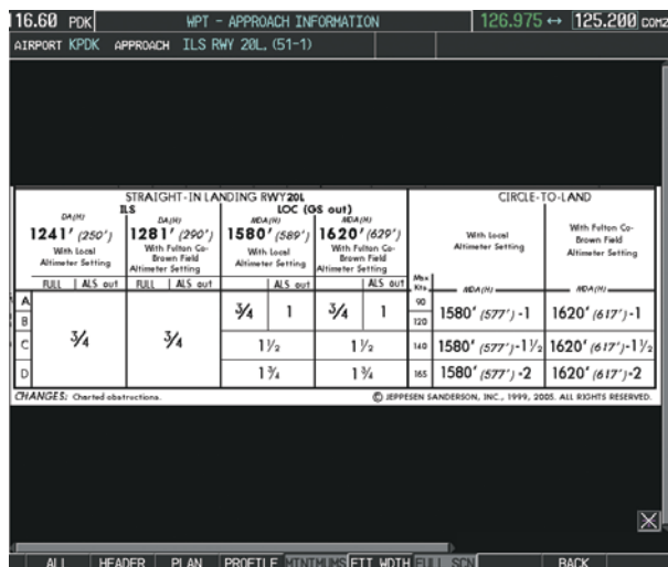
Figure 11-21 Approach Information Page, Minimums View
