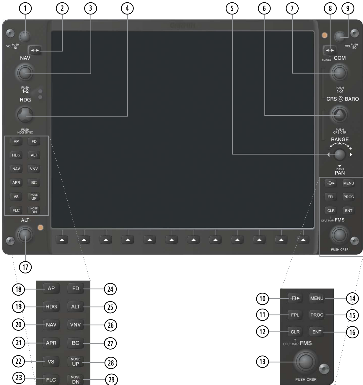
Figure 1-1 PFD/MFD Controls
