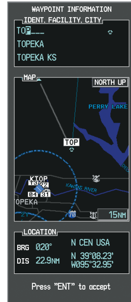
Figure 7-14 Entering V4 Entry Point
