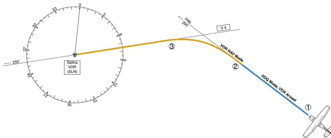
Figure 6-32 Intercepting a VOR Radial
