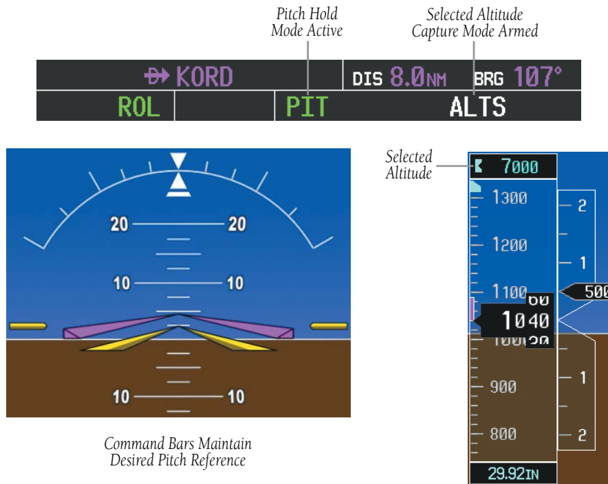
Figure 6-5 Pitch Hold Mode
