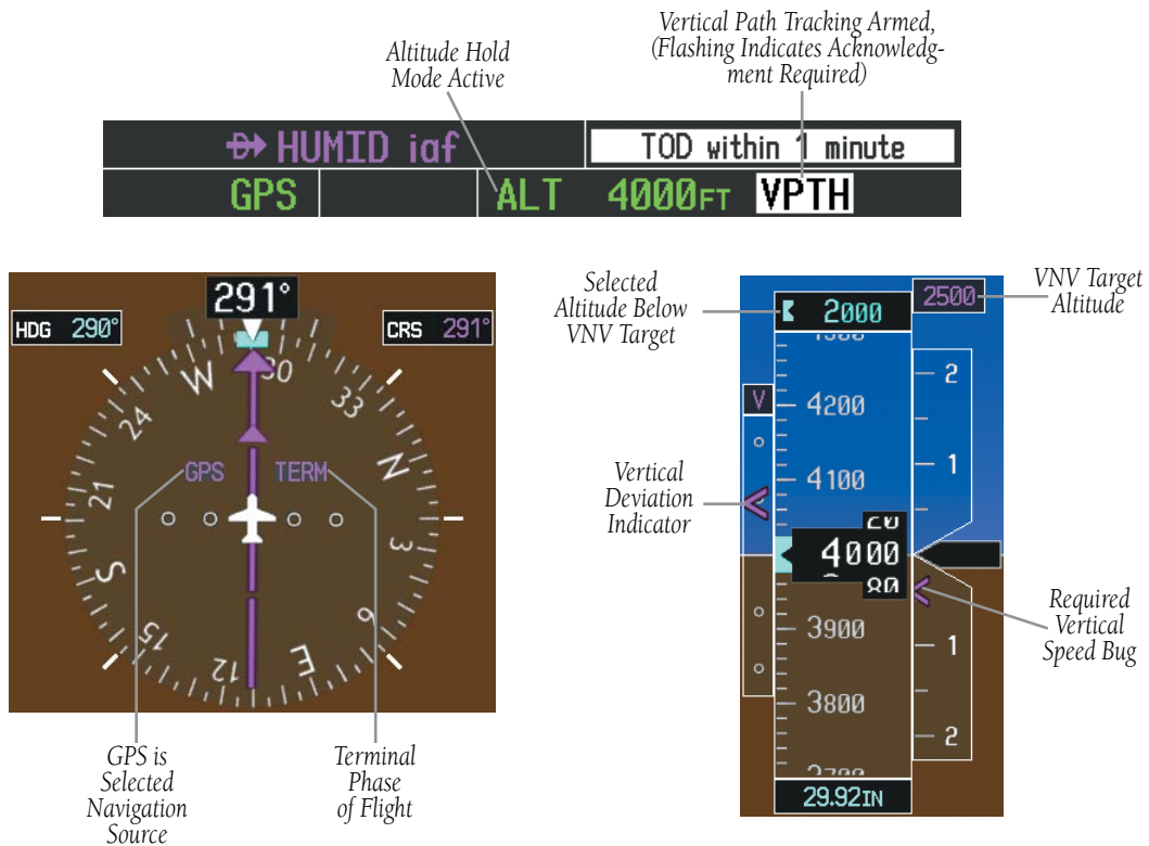
Figure 6-11 Vertical Path Capture
